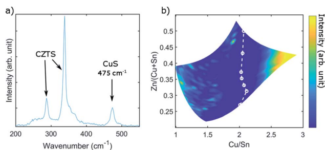
Fig. 2 (a) Raman spectrum (532 nm excitation) with CZTS Raman modes in the range 250–400 \text{cm}^{-1} . CuS mode visible at 475\text{ cm}^{-1} . (b) Integrated intensity in the region of the CuS peak against the cation composition from EDX. The phase boundary for CuS is marked with a white dashed line.
