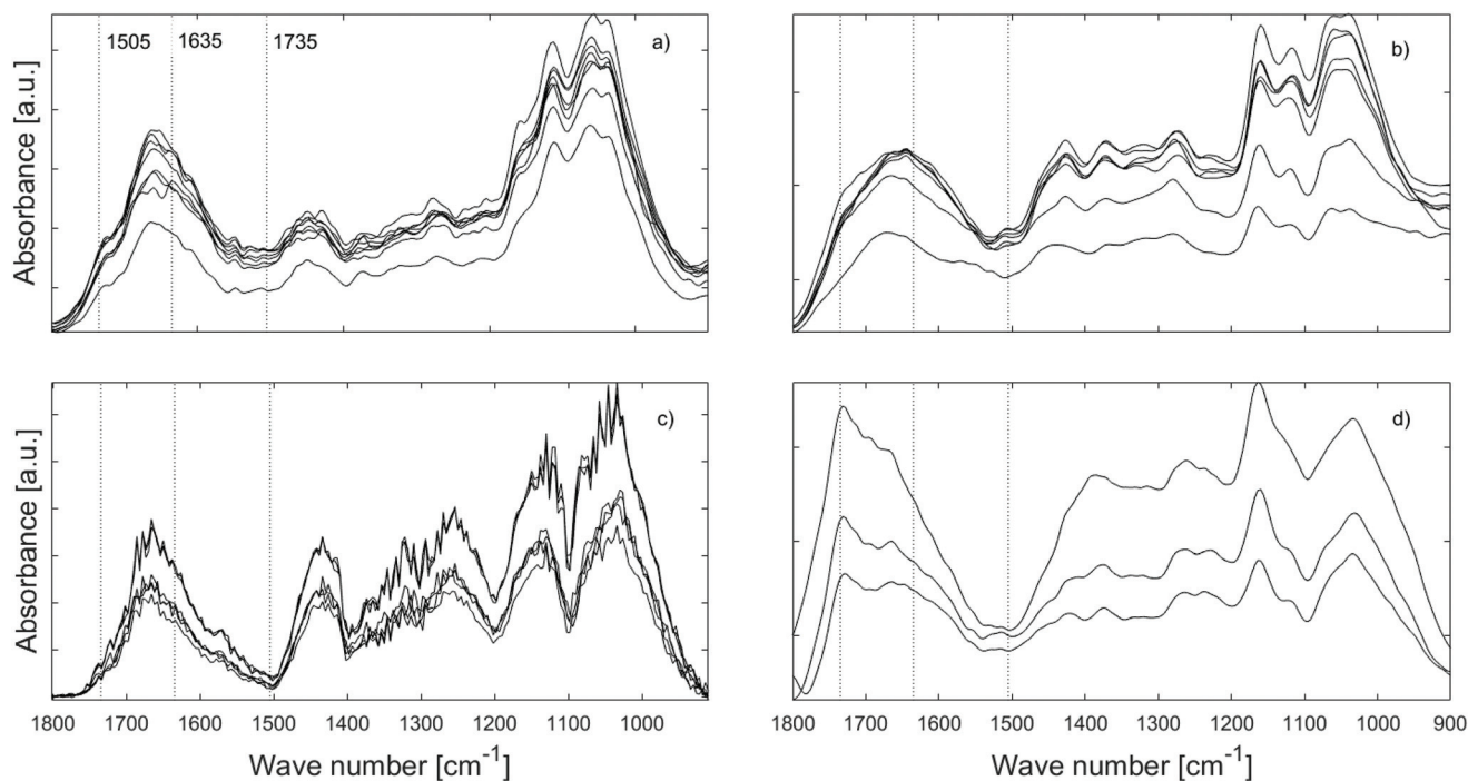
Fig. 6 AFM-IR spectra of gribble faecal pellets (feeding trial 1, treatment 2) obtained after 7 (a) and 28 days (b) of feeding on untreated wood, and 7 (c) and 28 days (d) of feeding on furfurylated wood.
