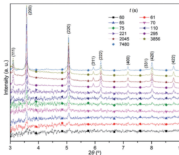
Fig. 10 (Fig. 3 from ref. 108). XRD patterns taken from the reaction mixture containing KBr and NaCl with a molar ratio [\text{KBr}]/([\text{NaCl}] + [\text{KBr}]) = 4/8 used for the synthesis of AgCl _x Br _{1-x} nanocubes (SEM image in Fig. 1 from ref. 108). Different patterns were recorded at different times normalized against time when the AgNO _3 solution was injected into the reaction mixture. Injected into the 12 mL ethylene glycol solution of 0.35 mmol NaCl and 0.70 mmol KBr plus 2.5 g polyvinylpyrrolidone (PVP) was a 1.0 mL ethylene glycol solution of AgNO _3 (0.34 M) at an injection rate of 1 mL min ^{-1} with the assistance of a syringe pump. The X-ray wavelength was 0.1771 Å. Reproduced with permission from ref. 108. Copyright 2015 Royal Society of Chemistry.
