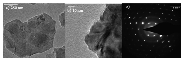
Fig. 2 TEM images (a) and (b). Diffraction of DPCOF spacing which corresponds to 2\theta 18–19°. The CTM image displays clear hexagonal symmetry and crystalline order which can be seen in DPCOF SAD (c) diffraction from (b).
