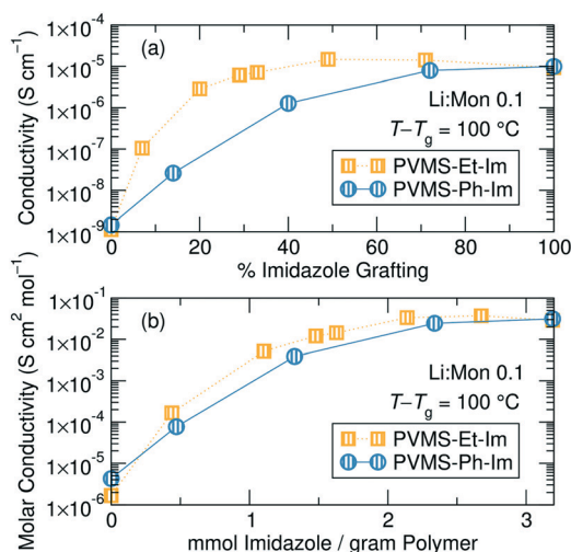
Fig. 5 (a) T_g -normalized total ion conductivity versus grafting density for the ethane-imidazole and phenyl-imidazole polymer series at a Li + :monomer ratio of 0.1. (b) The T_g -normalized conductivity can be approximately normalized by salt concentration (to obtain molar conductivity) and plotted against the mmol of imidazole per gram polymer which acts as a proxy for imidazole molar volume. These data now show a very similar trend between the ethane and phenyl series. Error bars are smaller than symbols.
