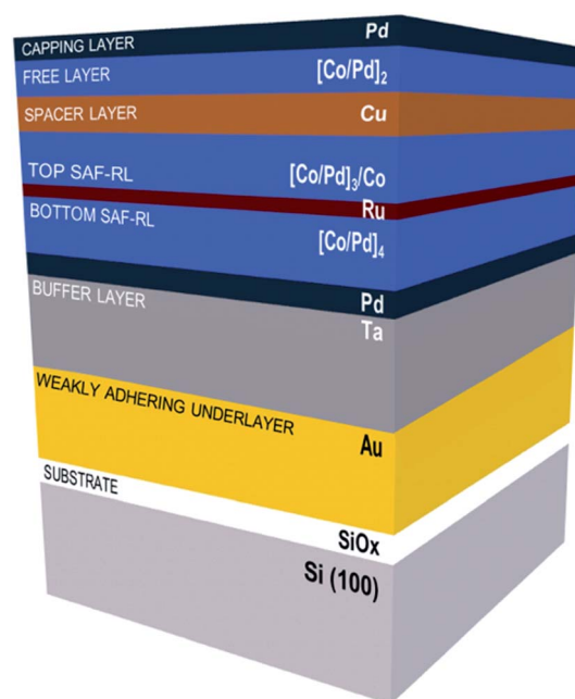
Fig. 1 Schematic sample structure of the Co/Pd-based GMR-SV stack consisting of a [Co/Pd] 4 /Ru/[Co/Pd] 3 /Co synthetic antiferromagnet reference layer (SAF-RL) and a [Co/Pd] 2 free layer separated by a Cu spacer layer. Reference samples were directly deposited on SiO x /Si(100) substrates, while a weakly adhering Au underlayer was interposed to allow for the transfer of the stack on a flexible tape.
