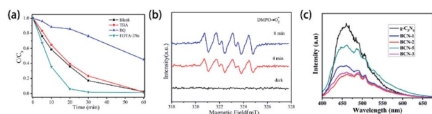
Fig. 10 (a) Species trapping experiments for the degradation of rhodamine B; (b) DMPO spin-trapping ESR spectra of P-Cl co-doped g-CN. Reprinted with permission from ref. 103, copyright 2020, Elsevier. (c) PL spectra of pristine g-CN and Ba-doped g-CN. Reprinted with permission from ref. 147, copyright 2020, Elsevier.
