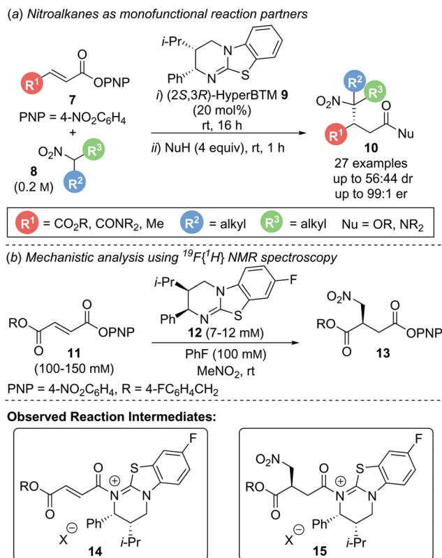
Scheme 4 (a) Aryloxide turnover in the conjugate addition of nitroalkanes; (b) mechanistic investigation.
