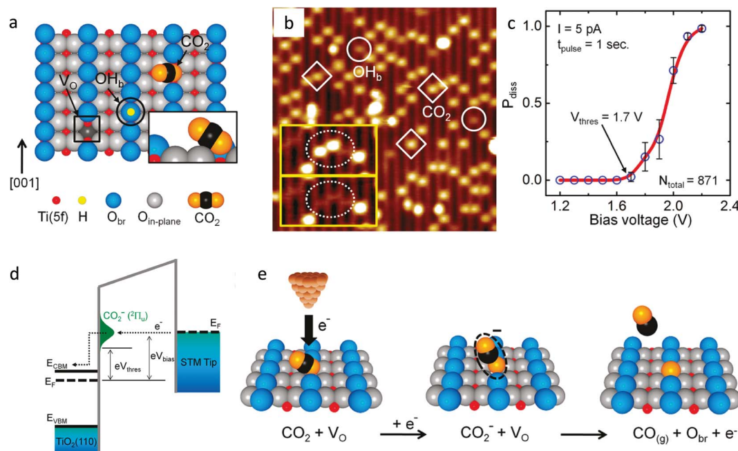
Fig. 4 (a) Schematic showing the oxygen vacancy ( \text{V}_\text{O} , in a black color square), bridged hydroxyl group ( \text{OH}_\text{b} , black color circle) and \text{CO}_2 molecule adsorbed at the \text{V}_\text{O} site on the reduced \text{TiO}_2 (1) (1 × 1) surface. The fivefold-coordinated \text{Ti}(5f) atoms and bridged oxygen ( \text{O}_\text{br} ) are indicated in red and blue, respectively. The inset shows that the molecular axis of \text{CO}_2 is perpendicular to the direction of the bridging-oxygen row ([001] azimuth) and is tilted away from the surface normal by 57°; (b) STM image (1.5 V, 5 pA, 15 nm × 15 nm) of the \text{TiO}_2 (110) surface after adsorption of \text{CO}_2 at 55 K. Three \text{CO}_2 and two \text{OH}_\text{b} features are shown as diamonds and circles, respectively. The inset shows two STM images (5.1 nm × 2.6 nm) of the same area on the surface. The upper inset shows two \text{CO}_2 molecules (in the dotted ellipse) that diffused away from their \text{V}_\text{O} sites, leaving two intact \text{V}_\text{O} sites visible, as shown in the lower inset image; (c) dissociation probability ( P_{\text{diss}} ) plotted as a function of bias voltage. The threshold voltage was V_{\text{thres}} = +1.7 V, and P_{\text{diss}} approached 1 at +2.2 V. (d) The electron-transfer process at the STM tip/ \text{CO}_2 / \text{TiO}_2 interface. Above eV_{\text{thres}} = 1.7 eV, the electrons start to tunnel into the negative-ion state of the adsorbed \text{CO}_2 and (e) schematics of an electron-induced \text{CO}_2 dissociation process (reproduced from ref. 44 with permission from the American Chemical Society, copyright 2011).
