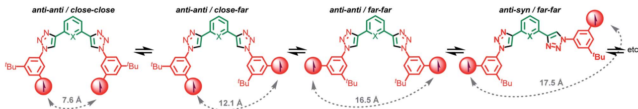
Scheme 2 Limiting main conformations of the bis(triazolyl)pyridines ( X = N ) and bis(triazolyl)phenyl ( X = CH ) axes. Calculated distances shown here refer to Axle-2 ( X = CH ).
