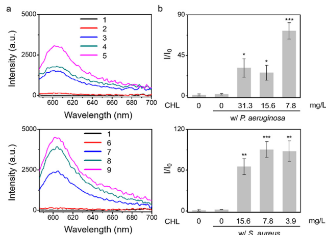
Fig. 2 TCF-OTf based fluorescence detection (a) and corresponding change in fluorescence (b) using P. aeruginosa and S. aureus without antibiotic treatment (control), and P. aeruginosa and S. aureus picked from the MIC plate wells under treatment at sub-MIC concentrations with chloramphenicol (CHL). 1, TCF-OTf; 2, P. aeruginosa with (w/) TCF-OTf; 3, P. aeruginosa + 31.3 mg L -1 CHL w/ TCF-OTf; 4, P. aeruginosa + 15.6 mg L -1 CHL w/ TCF-OTf; 5, P. aeruginosa + 7.8 mg L -1 CHL w/ TCF-OTf; 6, S. aureus w/ TCF-OTf; 7, S. aureus + 15.6 mg L -1 CHL w/ TCF-OTf; 8, S. aureus + 7.8 mg L -1 CHL w/ TCF-OTf; and 9, S. aureus + 3.9 mg L -1 CHL w/ TCF-OTf. * P < 0.02, ** P < 0.002, *** P < 0.001. \lambda_{\text{ex}} = 560 nm, \lambda_{\text{em}} = 606 nm.
