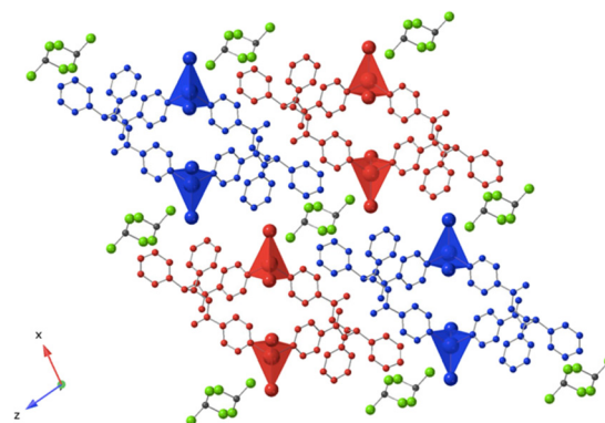
Fig. 6 Portion of the X-ray structure of \text{L-CdI}_2 showing the packing of consecutive 1D zig-zag type networks in the xOz plane. H atoms are not represented for clarity.
