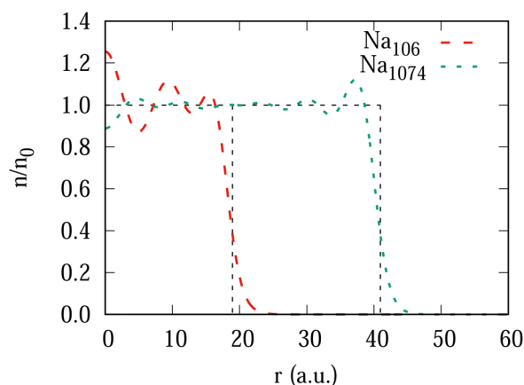
Fig. 9 Ground state electron density profile of the spherical clusters Na 106 and Na 1074 in the units of the constant background density n_0 (thin dashed line) as a function of the radial coordinate.
