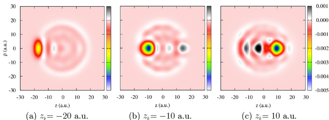
Fig. 10 Change of the electron density, \Delta n , of the Na 106 cluster (radius R_{cl} = 18.93 a.u.) upon collision with antiproton. The density change is defined as \Delta n(z, \rho, z_p) = n(z, \rho, z_p[t]) - n(z, \rho, z_p[t = 0]) . Results are shown as a function of the cylindrical ( z, \rho ) coordinates. The projectile moves with constant velocity v = 0.1 a.u. along the straight-line trajectory following the symmetry z -axis of the system that passes through the center of the cluster. The snapshots correspond to three different antiproton positions: (a) z_p = -20 a.u., (b) z_p = -10 a.u., (c) z_p = 10 a.u. The color code shows the density change in electrons per (a.u.) 3 .
