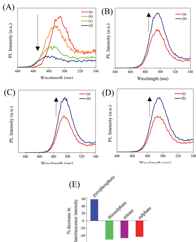
Fig. 4 (A) Emission spectrum of (a) Zn Au NCs in human blood serum and those following the addition of (b) 22.2 μL, (c) 32.2 μL and (d) 42.2 μL of pyrophosphate ions in human blood serum. (B) Emission spectrum of (a) Zn Au NCs in human blood serum and that following the addition of (b) 32.2 μL of sulphate ions in human blood serum. (C) Emission spectrum of (a) Zn Au NCs in human blood serum and that following the addition of (b) 32.2 μL of nitrate ions in human blood serum. (D) Emission spectrum of (a) Zn Au NCs in human blood serum and that following the addition of (b) 32.2 μL of thiosulphate ions in human blood serum. (E) Bar diagram showing the percentage decrease in luminescence intensity of Zn Au NCs upon the addition of pyrophosphate and various other interfering agents in human blood serum.
