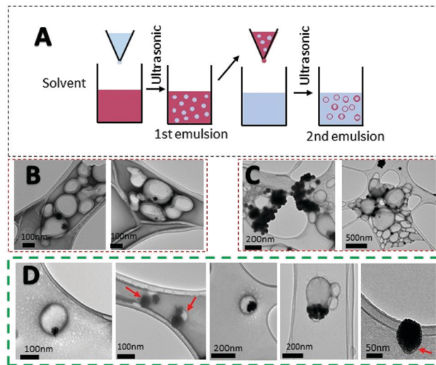
Fig. 6 Nanoemulsion encapsulation of PtNPs with PLGA particles. (A) Schematic illustration of the double emulsion process to form particles. TEM images of double emulsion encapsulation with three different concentrations of PtNPs (B) 0.01 \text{ mg } \mu\text{L}^{-1} (C) 0.02 \text{ mg } \mu\text{L}^{-1} (D) 0.015 \text{ mg } \mu\text{L}^{-1} . Concentration tested on (D) 0.015 \text{ mg } \mu\text{L}^{-1} resulted in the highest encapsulation rate of PtNPs, and therefore was used for further experiments.
