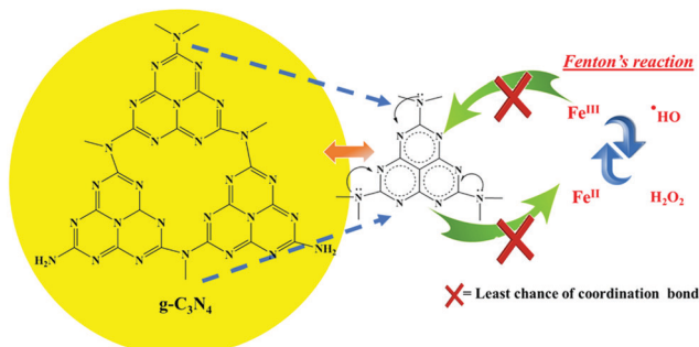
Fig. 8 (a) Alkaline stability of the QPS and QPS-CN x composite membranes in 3 M NaOH for 300 h and (b) the related mechanism showing the stability against Fenton's reagent.
