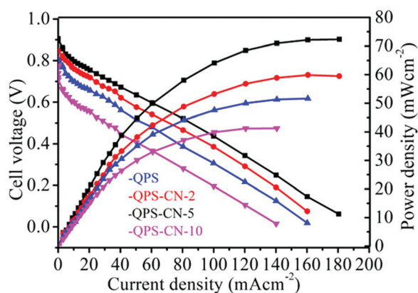
Fig. 9 Cell performance of the QPS and QPS–CNx composite membranes at a 300\text{ cm}^3\text{ min}^{-1} \text{H}_2/\text{O}_2 flow rate under 100% RH.
