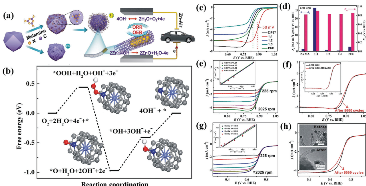
Fig. 12 (a) Schematic illustration of the synthetic strategy for Co@CNTs. (b) Free-energy diagram for the ORR on Co@CNTs in alkaline ( \text{pH} = 13 ) media. ORR activities of Co@CNTs in both alkaline and acidic media. (c) LSV curves and (d) J_K and E_{1/2} of Co@CNTs and other comparative catalysts in 0.1 \text{ M KOH} . (e) LSV curves of the Co@CNTs at different rotating rates. Inset: the K–L plot at various potentials. (f) LSV curves of Co@CNTs and the sample after 5000 cycles (the inset shows 0.1 \text{ M KOH} solution with and without 1 \text{ M} methanol). (g) LSV curves of Co@CNTs at different rotating rates in 0.5 \text{ M H}_2\text{SO}_4 . Inset: the K–L plot at various potentials. (h) LSV curves of Co@CNTs and the sample after 5000 cycles (inset: TEM images before and after 5000 cycles). MA: melamine; 1:1, 1:2 and 1:3 are the ratios of \text{weight}_{\text{ZIF-67}} : \text{weight}_{\text{melamine}} , respectively. Reproduced from ref. 257 with permission from Science Press and Dalian Institute of Chemical Physics, Chinese Academy of Sciences. Published by Elsevier B.V. and Science Press.
