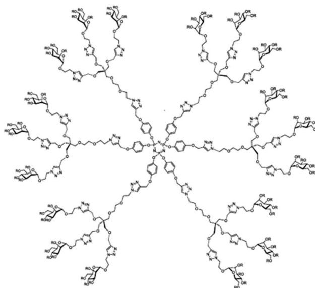
Fig. 26 (a) Structure of hetero-layered hybrid glyco-dendrimer (41). (b) Chemical structure of mannosylated dendrimer (42).
