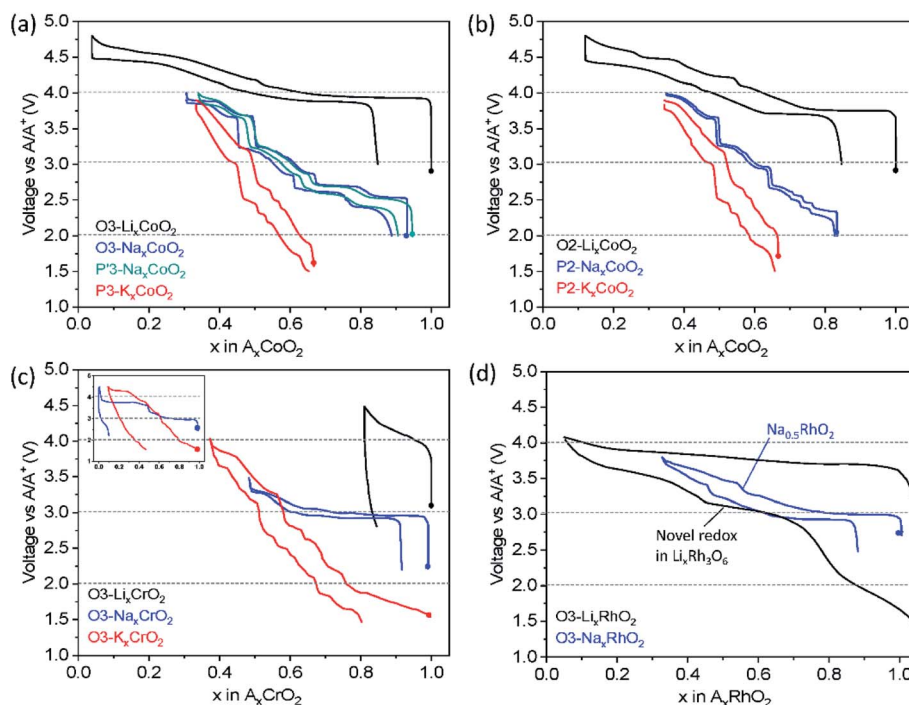
Fig. 5 Typical charge/discharge profiles of (a) O3 and P'13 type A_x\text{CoO}_2 , (b) O2 and P'12 type A_x\text{CoO}_2 , (c) O3 type A_x\text{CrO}_2 with an inset for those cycled in higher upper cut-off voltage, and (d) O3 type A_x\text{RhO}_2 in non-aqueous Li, Na, and K cells. Filled circle represents a starting point of charge.
