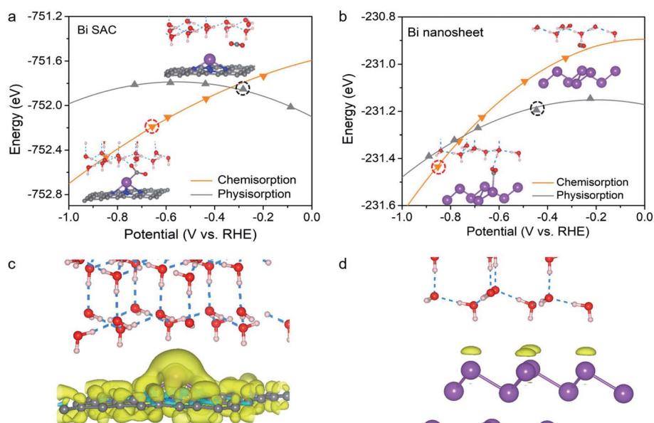
Fig. 2 Calculated total energies of chemisorbed CO 2 (*CO 2 ) and physisorbed CO 2 of (a) the Bi–N–C SAC and (b) the Bi nanosheets as a function of potential U . Charge density difference for (c) the Bi–N–C SAC and (d) the Bi nanosheets when the applied potential changes from 0 to –0.6 V. The iso-value is 0.0006 a.u.
