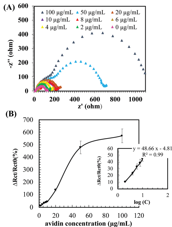
Fig. 7 (A) Impedance Nyquist plots of the EIS from ITO modified with PG/b-pSBAE ( 8/30 \text{ mg mL}^{-1} ) after immersion in avidin solution at various concentrations ( 0\text{--}100 \mu\text{g mL}^{-1} ). Measurements were performed in PBS containing 10 \text{ mM } [\text{Fe}(\text{CN})_6]^{3-/4-} and 0.1 \text{ M KCl} . (B) Changes in the charge transfer resistance [ \Delta R_{ct}/R_{ct0} (%)] of the PG/b-pSBAE modified ITO after immersion in avidin solution at various concentrations. Insert: the corresponding regression curve of the PG/b-pSBAE modified ITO. C: Avidin concentration. Value = mean \pm standard deviation, n = 3 .
