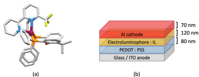
Fig. 11 (a) Structure of the [\text{Cu}(\text{xanthos})(6\text{-CF}_3\text{bpy})]^+ cation in the [\text{PF}_6]^- salt (CSD refcode VICQUW); the 6- \text{CF}_3 bpy ligand is disordered over two sites and only the major occupancy site is shown. H atoms are omitted. (b) Architecture of LECs containing the Cu-iTMCs with \text{CF}_3 -functionalized bpy ligands. IL = [\text{EMIM}][\text{PF}_6] and Cu-iTMC: IL molar ratio = 4 : 1. LECs were driven using a pulsed current.
