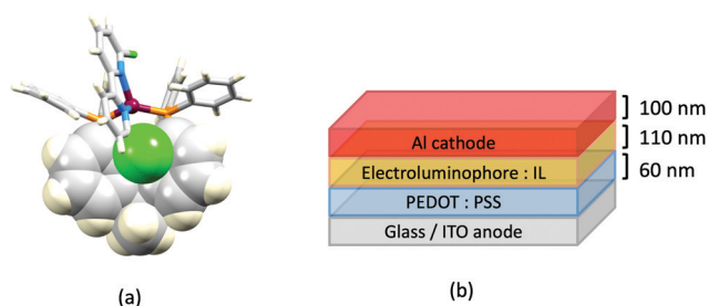
Fig. 10 (a) Structure of the cation in [Cu(xantphos)(6,6'-Cl 2 bpy)]PF 6 (CSD refcode MEWXUK). (b) Architecture of LECs containing the Cu-ITMCs with halogen-substituted bpy ligands. IL = [EMIM][PF 6 ] and Cu-ITMC: IL molar ratio = 4 : 1. LECs were driven using a pulsed current.
