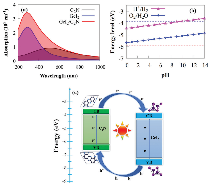
Fig. 6 (a) Calculated absorption spectra of the 2 \times 2 supercell of C_2N , the 4 \times 4 supercell of GeI_2 and the GeI_2/C_2N vdW heterostructure. (b) The absolute energy bands for the conduction band minimum and valence band minimum of the GeI_2/C_2N vdW heterostructure with respect to pH (0–14). (c) Schematic diagram showing the transfer of photogenerated electrons and holes.
