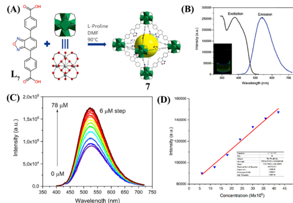
Fig. 4 (A) Synthesis of sensor LMOF 7 from ligand L7 and Zr(IV); (B) Excitation and emission spectra of 7 were measured in H 2 O (inset: photographs of 7 in H 2 O); (C) Changes in fluorescence emission intensity for 7 upon the gradual addition of aqueous NH 3 . (D) Linear fit for the NH 3 concentration–intensity correlation. Reprinted with permission from ref. 51. Copyright 2022 Royal Society of Chemistry.
