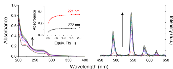
Fig. 1 Changes in (left) UV-Vis absorption and (right) phosphorescence spectra of an aqueous solution of 3Gal on addition of \text{Tb}(\text{CF}_3\text{SO}_3)_3 . Inset: Binding isotherms.
