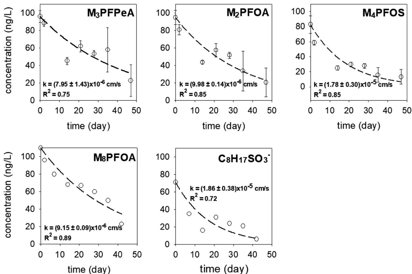
Fig. 5 The concentration–time profile of the PRCs in the samplers deployed in the sediment at Lake Niapenco in October 2021 ( M_3 PFPeA, M_2 PFOA, and M_4 PFOS) and June 2022 ( M_8 PFOA and C_8H_{17}SO_3^- ).
