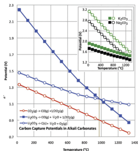
Fig. 5 Electrochemical conversion potential for carbon capture and conversion centra \text{Li}_2\text{CO}_3 (main figure), or \text{Na}_2\text{CO}_3 or \text{K}_2\text{CO}_3 (figure inset); in the inset, squares refer to \text{M}_2\text{CO}_3 \rightarrow \text{C} + \text{M}_2\text{O} + \text{O}_2 and circles to \text{M}_2\text{CO}_3 \rightarrow \text{CO} + \text{M}_2\text{O} + \frac{1}{2} \text{O}_2 . To the right of the brown vertical line, CO is preferred. And C is preferred to the left of the line. 74
