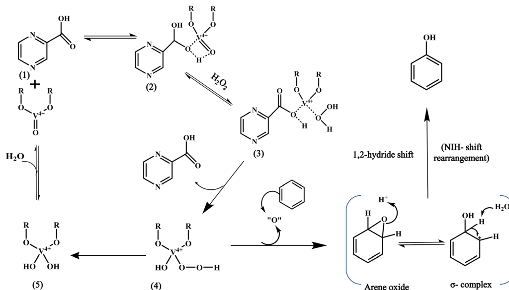
Scheme 21 Proposed reaction mechanism for the formation of vanadium-PCA complex in \text{H}_2\text{O}_2(\text{aq}) - \text{CH}_3\text{CN} system ( \text{R} = bulk \text{VO}_x ).
