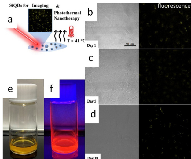
Fig. 17 Photothermal nano therapy of 10-undecanoic acid functionalized SiQD. (a) Cartoon representation of Photothermal nanotherapy of SiQDs photoimaging. (b)–(d) fresh and aged SiQDs fluorescence. (e) and (f) Colloidal SiQDs under visible and UV light. Adapted with permission from ref. 140. Copyright (2022) American Chemical Society.
