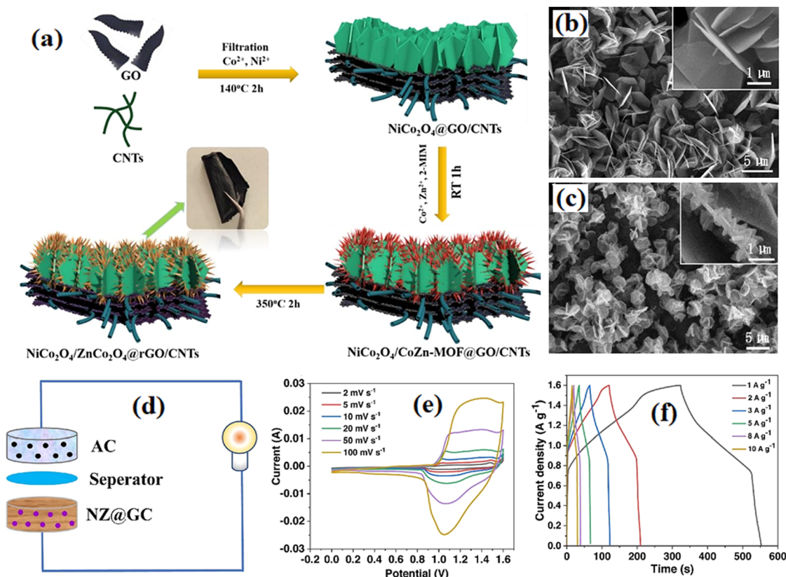
Fig. 7 (a) Fabrication process of NiCo 2 O 4 /ZnCo 2 O 4 @rGO/CNTs. (b) SEM image of NiCo 2 O 4 @GO/CNTs. (c) SEM image of NiCo 2 O 4 /ZnCo 2 O 4 @rGO/CNTs film. (d) Assembly illustration of the NZ@GC//AC hybrid supercapacitor. (e) CV and (f) GCD curves of the supercapacitor. 127
