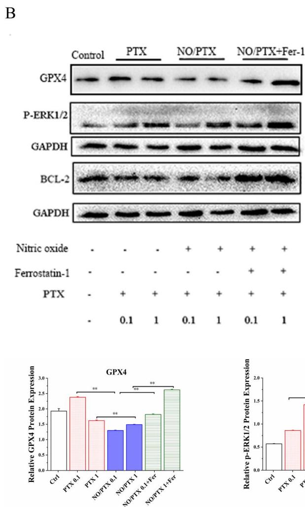
Fig. 4 (A) The intracellular GSH-Px, MDA and SOD levels in the cells treated with PTX, NO/PTX or NO/PTX + Fer-1 ( *P < 0.05 , **P < 0.01 ). (B) Expression of ferroptosis-related proteins in the cells treated with PTX, NO/PTX or NO/PTX + Fer-1 ( **P < 0.01 ).
