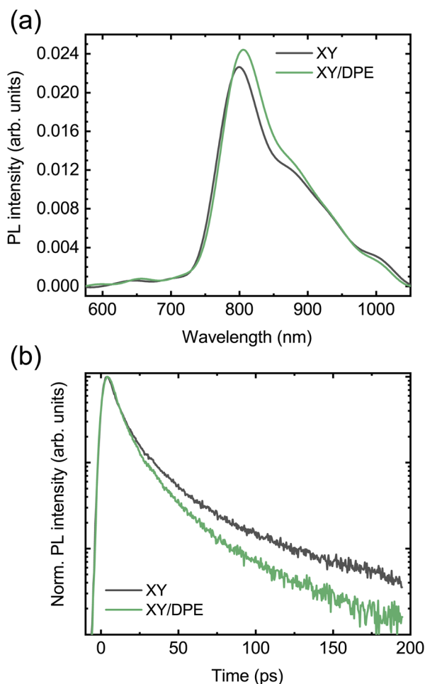
Fig. 6 Photoluminescence measurements on TPD-3F:IT-4F blend films cast with and without the use of DPE: (a) steady-state photoluminescence; (b) decay of the PL signal at 800 nm.
