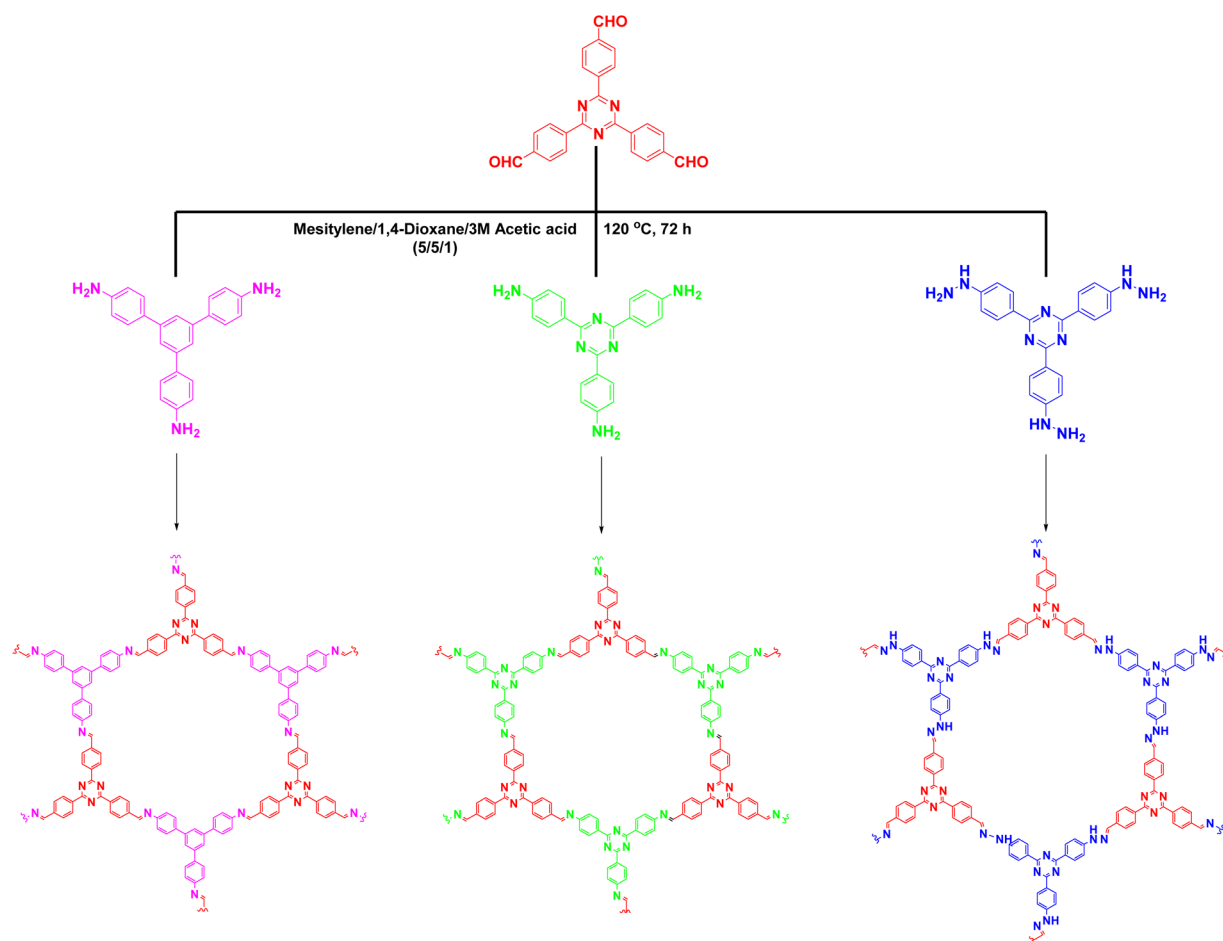
Fig. 10 COFs were synthesized by reaction of different nitrogenous building blocks with 4,4',4''-(1,3,5-triazine-2,4,6-tryl) Schiff bases.
