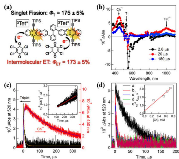
Fig. 18 (a) Schematic diagram of intermolecular electron transfer from iSF of tetracene dimer 14 to chloranil. (b) μs-TA spectra of dimer 14 (50 μM) in the presence of 250 μM chloranil in Ar-saturated PhCN after excitation at 532 nm. (c) Corresponding time profiles at 450 and 520 nm. The inset shows the second-order plots. (d) Time profiles of absorption at 520 nm in the presence of different concentrations of chloranil: (a) 0 mM, (b) 0.25 mM, (c) 0.53 mM, (d) 0.63 mM, and (e) 0.72 mM. The inset shows the plot of the pseudo-first-order rate constant (k obs ) vs. the concentration of chloranil. Reproduced with permission. 75 Copyright 2019, the American Chemical Society.
