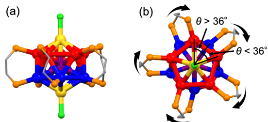
Fig. 1 (a) Side and (b) top view of the chiral structure of \text{MAu}_{12}\text{-dppe} ( \text{M} = \text{Ir}, \text{Au} ). Color code: yellow, Au on the \text{Cl-Au-M-Au-Cl} axis; red and blue, Au in the \text{Au}_5 rings; purple, M; orange, P; light green, Cl; gray, C.
