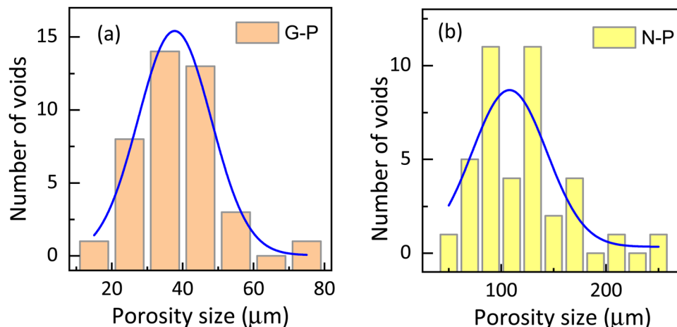
Fig. 6 Histogram showing the porosity size distribution in (a) gel-polymerized and (b) nematic polymerized samples (calculated from the SEM) images shown in Fig. 4(a) and (e). It should be noted that the horizontal scale is significantly different.
