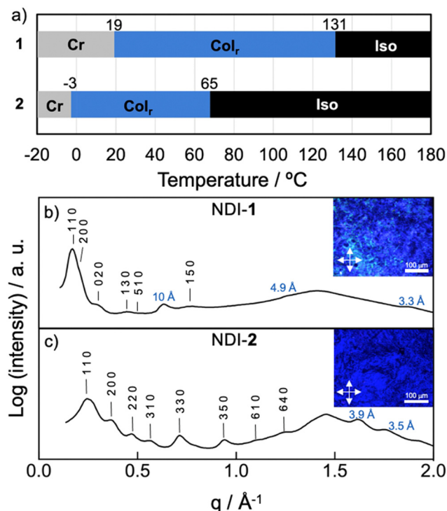
Fig. 3 (a) Temperature-dependent phase transition behaviour of NDIs 1 and 2 . Cr = crystal (according to POM observations); Col r = columnar rectangular; Iso = isotropic liquid. Phase-transition temperatures were obtained from the first cooling cycle of the DSC curves (Fig. S17 and S18, ESI†) and POM observations. (b) X-ray pattern of NDI- 1 at 100 °C indexed to a LC Col r phase ( a = 60 Å; b = 43 Å). Inset shows the POM image at 100 °C. (c) X-ray pattern of NDI- 2 at 60 °C indexed to a LC Col r phase ( a = 35 Å; b = 41 Å). Inset shows the POM image at 60 °C. Distances displayed in blue correspond to meridional signals (layer lines “ L = 1, 2, 3, \dots ”).
