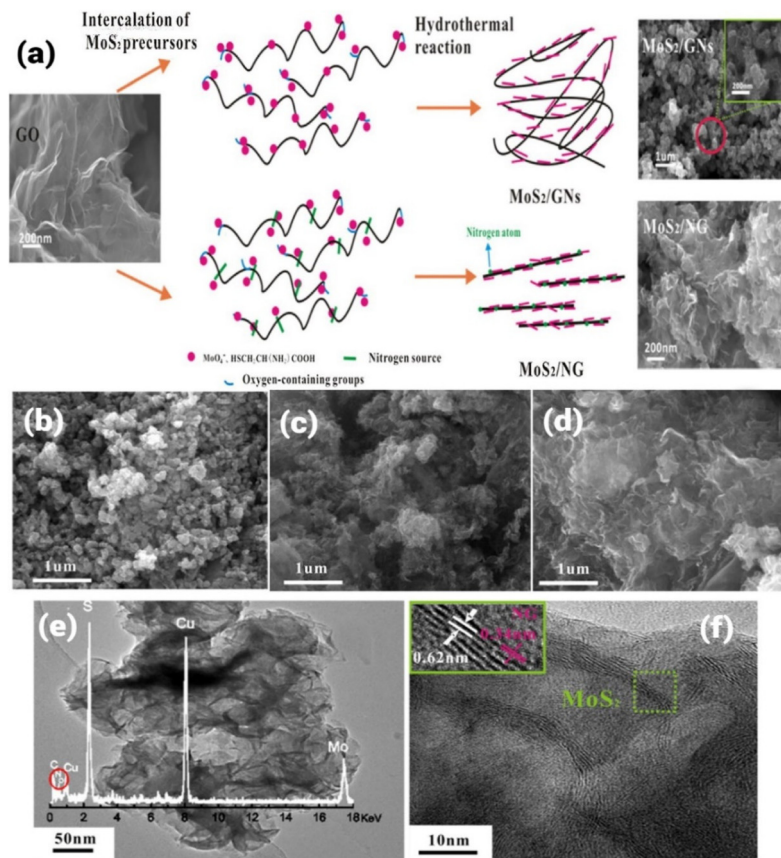
Fig. 3 (a) Schematic representation of the synthesis of \text{MoS}_2/\text{NG} and \text{MoS}_2/\text{graphene} nanosheet hybrids using typical hydrothermal approach, (b–d) SEM micrographs at 1.5:1, 3:1 and 5:1 ratio of \text{Na}_2\text{MoO}_4:\text{GO} respectively, and (e) TEM and (f) HRTEM micrographs of \text{MoS}_2/\text{NG} at 1.5:1 \text{Na}_2\text{MoO}_4:\text{GO} ratio. Reprinted with a permission from Reference (76). Copyright 2016, Elsevier.
