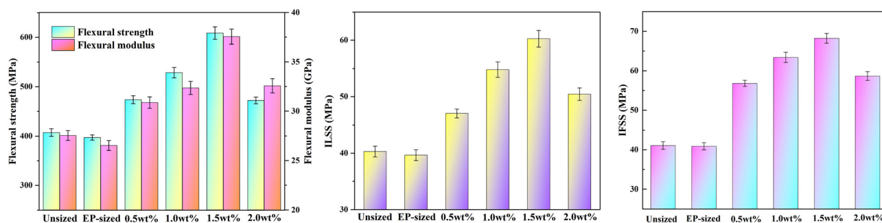
Fig. 4 Flexural strength, ILSS and IFSS values of different CF/PA6 composites.
