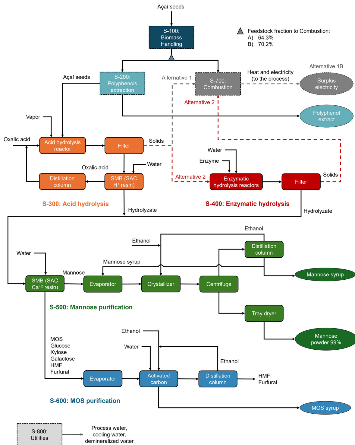
Fig. 1 Block flow diagram of biorefinery alternatives for processing açai seeds into mannose in powder and syrup form, MOS syrup, and polyphenol extract. SMB: simulated moving bed chromatography; SAC: strong acid cation exchange resin.
