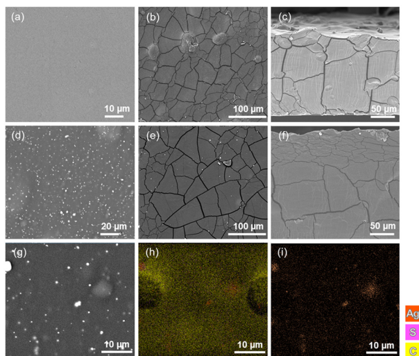
Fig. 5 Morphology characterization using SEM-EDX. SEM images of a) [AGR]_n film; b) [PS]_n film; c) cross section of [PS]_n film; d) 1^{(5\%)}@[AGR]_n , where CPs particles can be seen throughout at surface of the material; e) 1^{(5\%)}@[PS]_n ; f) cross section of 1^{(5\%)}@[PS]_n ; g) 1^{(5\%)}@[AGR]_n with h) an EDX analysis of Ag, C, and S distribution and i) the same section with silver distribution. Images were obtained at various magnifications: g), h), and i) 2000 \times ; a) 1200 \times ; d) 500 \times ; b) and e) 200 \times ; c), f) 160 \times .
