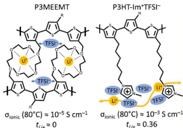
Fig. 35 Chemical structures for poly(3-(methoxyethoxyethoxymethyl)thiophene) (P3MEEMT) and poly(3-(6'-( N -methylimidazolium)hexyl)thiophene) (P3HT-Im + TFSI - ) used in the study. Reproduced from ref. 215 with permission from ACS, Copyright [2022].
