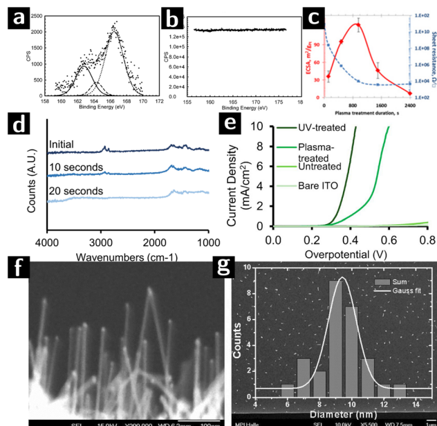
Fig. 7 Research on using plasmas to create heterogeneous catalysts from colloidal nanocrystals. (a) S 2s XPS spectra of Au@Pt nanoparticles (Pt/Au = 0.39) before and (b) after argon plasma treatment for 2 minutes. (c) ECSA values (red) and lateral electrical sheet resistance values (blue) at various RF argon plasma treatment durations of Au@Pt nanoparticles (Pt/Au = 0.39). 111 (d) FTIR spectra of a [Ni,Fe]O (Ni : Fe 51 : 49) nanoparticle film spin-coated on high resistivity Si (~10 \Omega -cm) after 0 s, 10 s or 20 s of air plasma treatment, at 0.2 torr. (e) Voltammograms of UV-treated, plasma-treated, untreated electrodes (functionalized with 51 : 49 [Ni,Fe]O nanoparticles), and a nanoparticle-free ITO control, in 0.1 M KOH. 112 (f) SEM image of SiNWs catalyzed by Au-apo, immobilized on a Si (111) substrate after O 2 -plasma treatment. (g) SEM image and the size distribution of 25 randomly selected SiNWs with unspecific growth directions.
