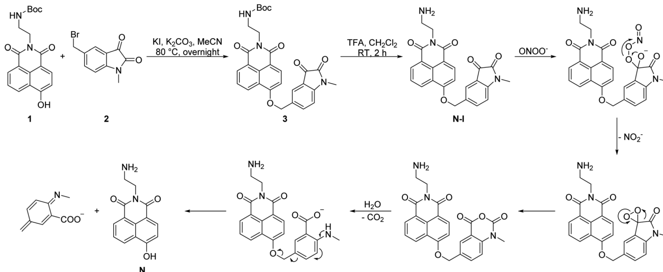
Scheme 2 The synthetic route of N-I and its proposed reaction mechanism with ONOO - .
