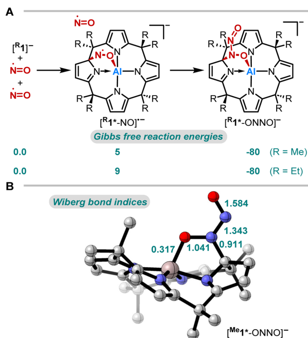
Fig. 3 (A) Computed Gibbs free reaction energies (kJ mol –1 ) for the reaction of [\mathbf{R}\mathbf{1}] with NO at the RI-DSD-PBEB95-D3(BJ)/def2-QZVPP, COSMO-RS( \text{CH}_2\text{Cl}_2 )/PBEh-3c level of theory and (B) Wiberg bond indices of [\text{Me}\mathbf{1}^*\text{-ONNO}]^- (PBE0/def2-TZVPP).
