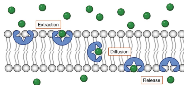
Fig. 2 Schematic representation of the anion transport mechanism by a synthetic carrier, consisting of the extraction of the anion from the aqueous environment into the lipid bilayer, the diffusion of the complex across the membrane, and the release of the anion on the other side.
