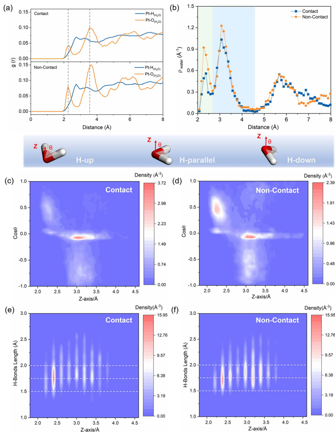
Fig. 2 (a) RDF of Pt-H(H 2 O) and Pt-O(H 2 O); (b) distribution of water number density and its proportion across different ranges; the two-dimensional density profile of the cos θ of H 2 O molecules in the contact (c) and non-contact (d) structures; two-dimensional density distribution profiles of H-bond lengths in the contact (e) and non-contact (f) structures.
