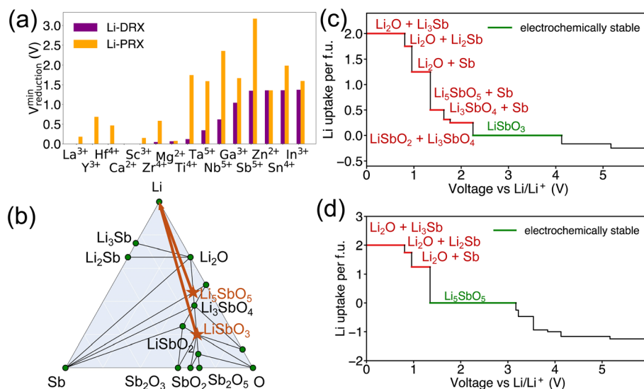
Fig. 2 (a) The minimum reduction voltage of Li-DRX and Li-PRX, and (b) the phase diagram of Li–Sb–O shows stable phases in green circles, the targeted compounds are marked as orange stars, and the orange arrows show the Li decomposition pathway of \text{LiSbO}_3 and \text{Li}_5\text{SbO}_5 . (c and d) The equilibrium voltage profiles and phase equilibria for lithiation reactions of the interface reactions at the anode/electrolyte of \text{LiSbO}_3 and \text{Li}_5\text{SbO}_5 respectively, the decomposition products of lithiation reactions at the anode side are labeled in red color, and the electrochemically stable voltage range is marked in green color.
