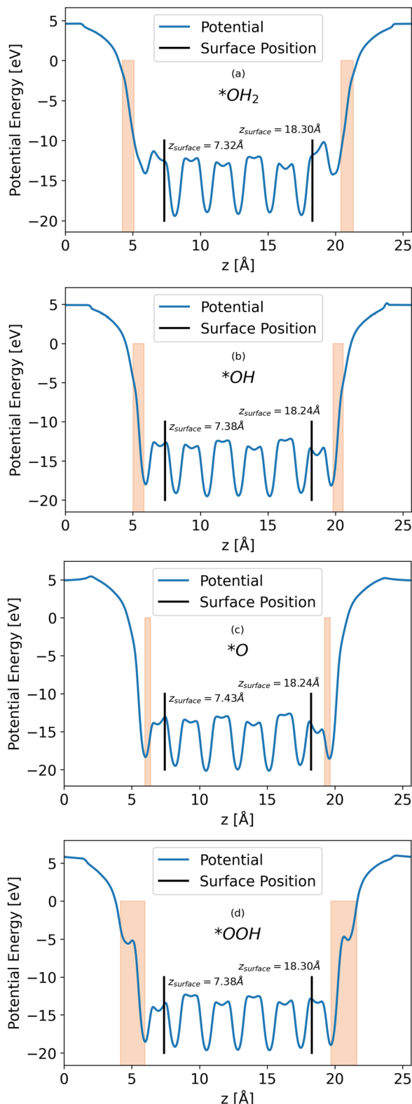
Fig. 2 x - y averaged potential of the (a) ^*\text{OH}_2 , (b) ^*\text{OH} , (c) ^*\text{O} , (d) ^*\text{OOH} intermediates (from top to bottom, respectively). The black lines in each graph represents the location of the bottom and top surfaces of the slab. Intermediate positions are shown in the orange shade.
