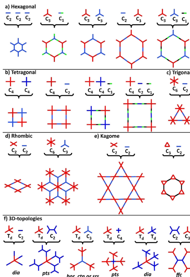
Fig. 2 Illustrative topology diagrams of common 2D and 3D-COFs.
